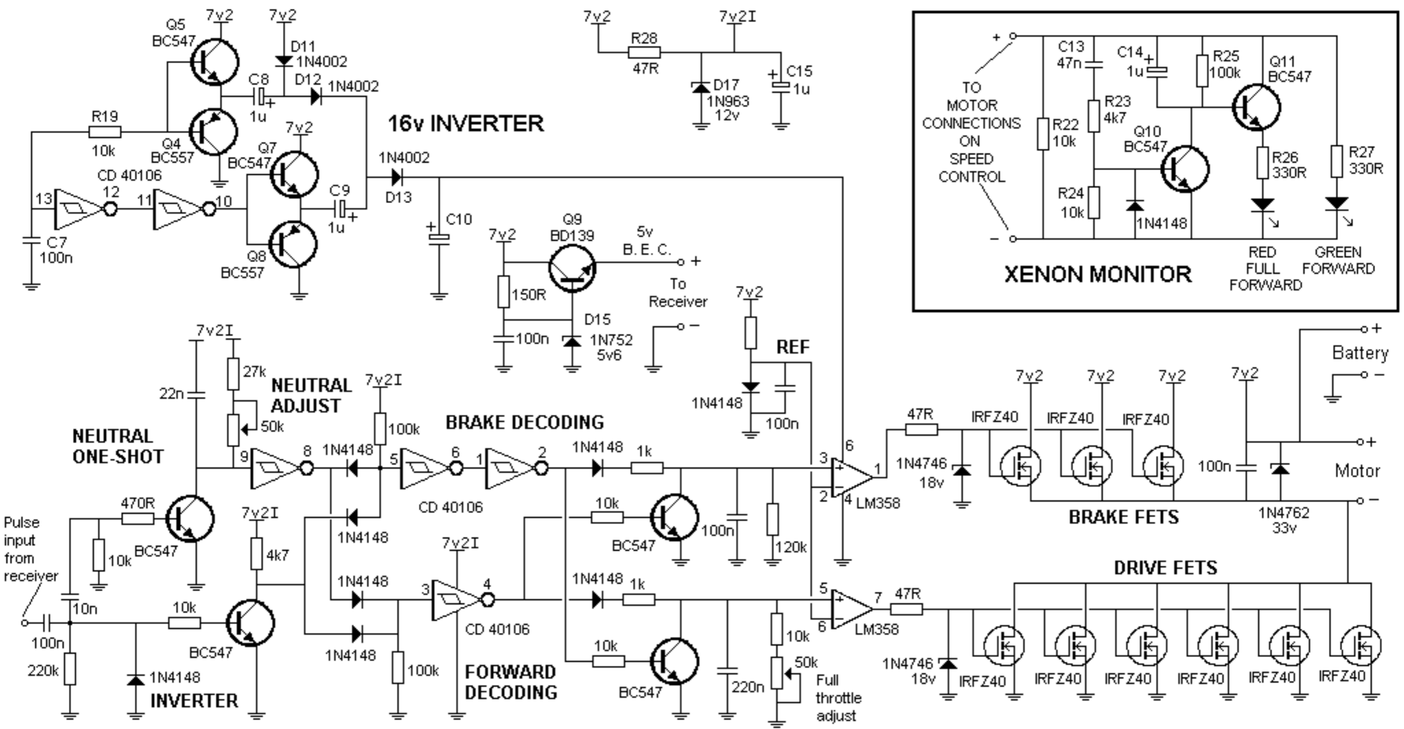
XENON 9 MOSFET SPEED CONTROLLER
